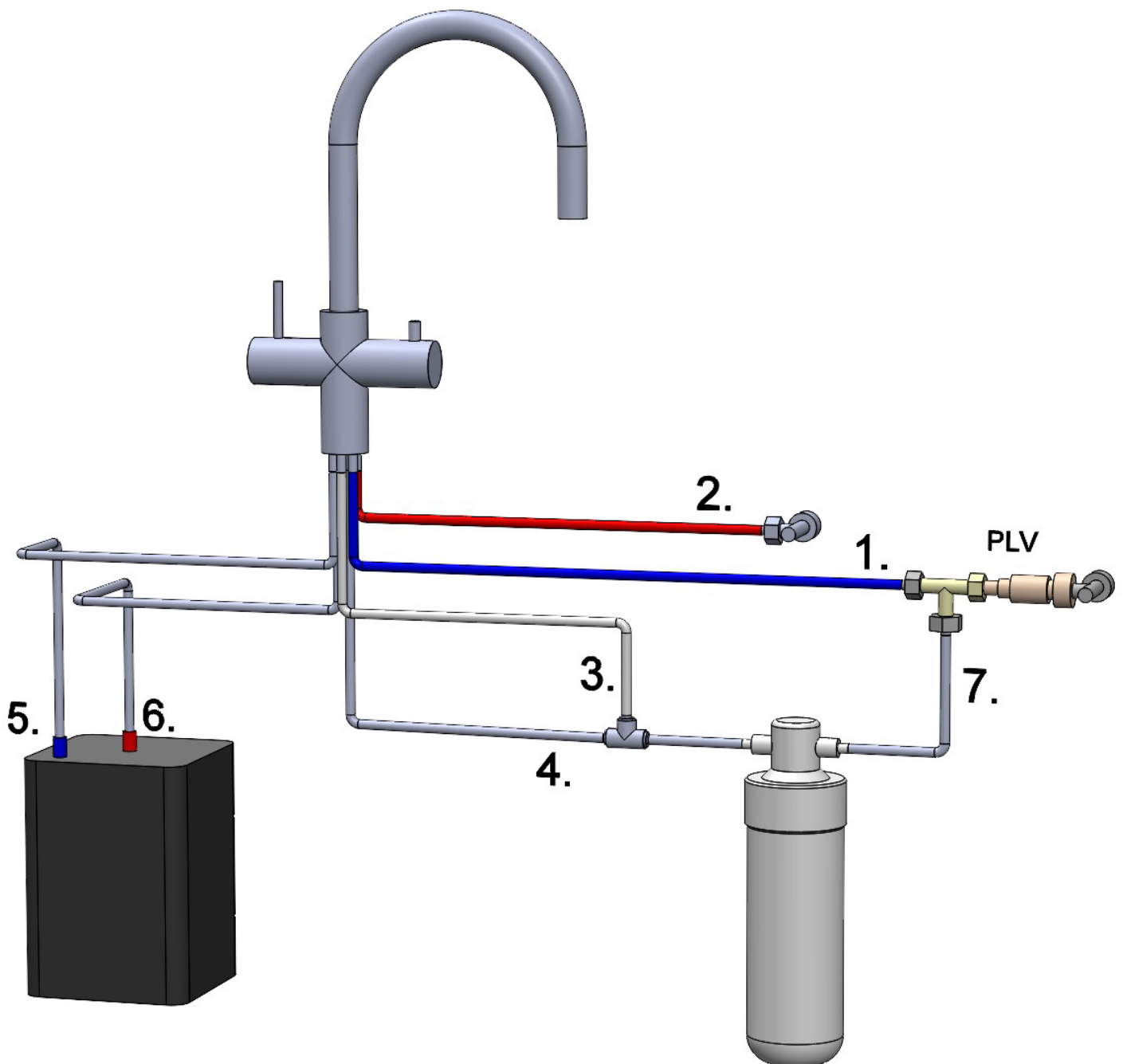
4in1 – REAR 3D VIEW
